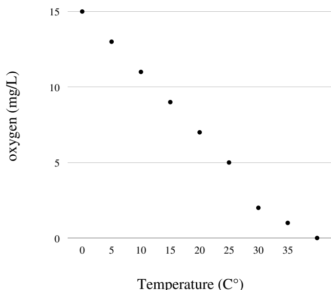
Figure 1: Solubility of Oxygen with temperature
